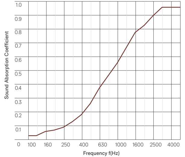
Sound Absorption Coefficients according to ISO 354. University of Auckland Testing Service Composition 10 - 12 mm - Test No. T0814-2b.
