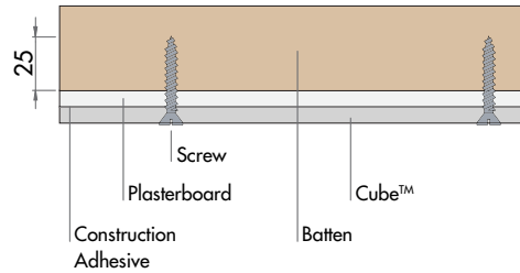
CUBE™ FIXED TO CEILING SUBSTRATE
