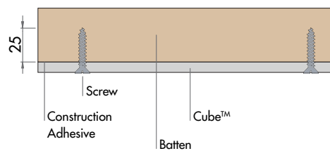
CUBE™ FIXED TO CEILING BATTENS
